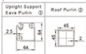
Profile Specifications
