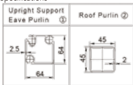
Profile Specifications
