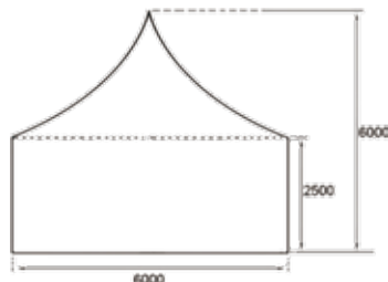
Gable Drawing
