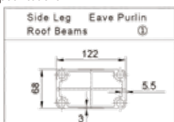
Profile Specifications
