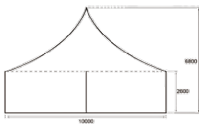
Gable Drawing
