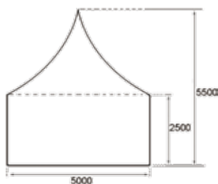
Gable Drawing
