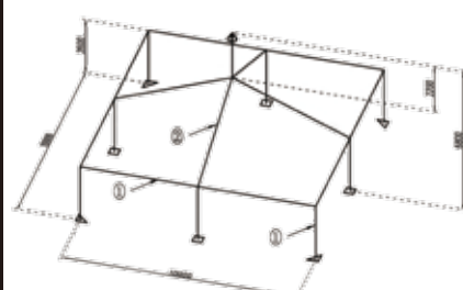
Frame Drawing
